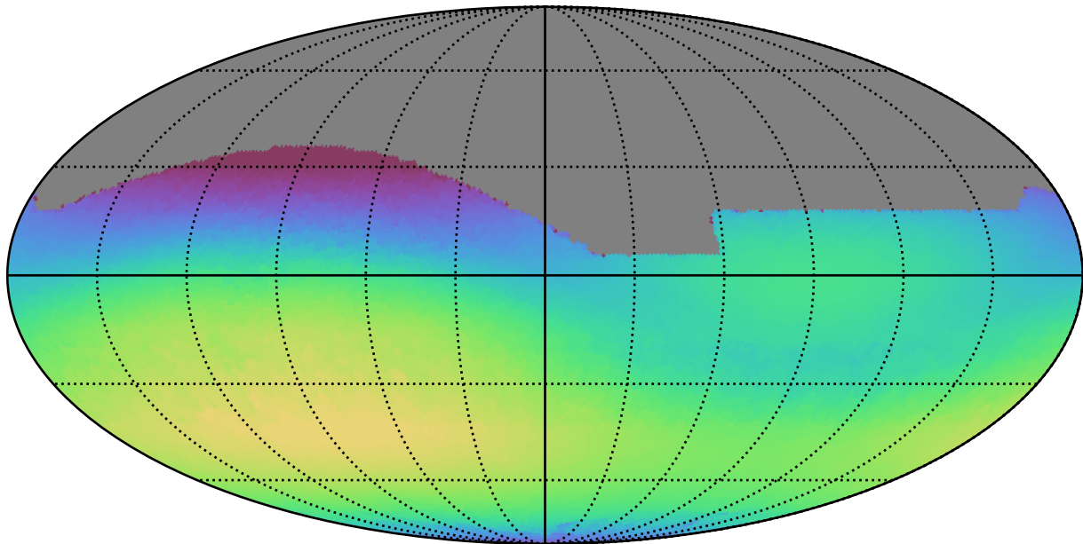
too_elab_r8_d2_giz_v3.4_10yrs All sky r band: Max skyBrightness
