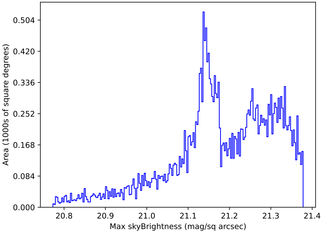
too_elab_r8_d2_giz_v3.4_10yrs All sky r band: Max skyBrightness
