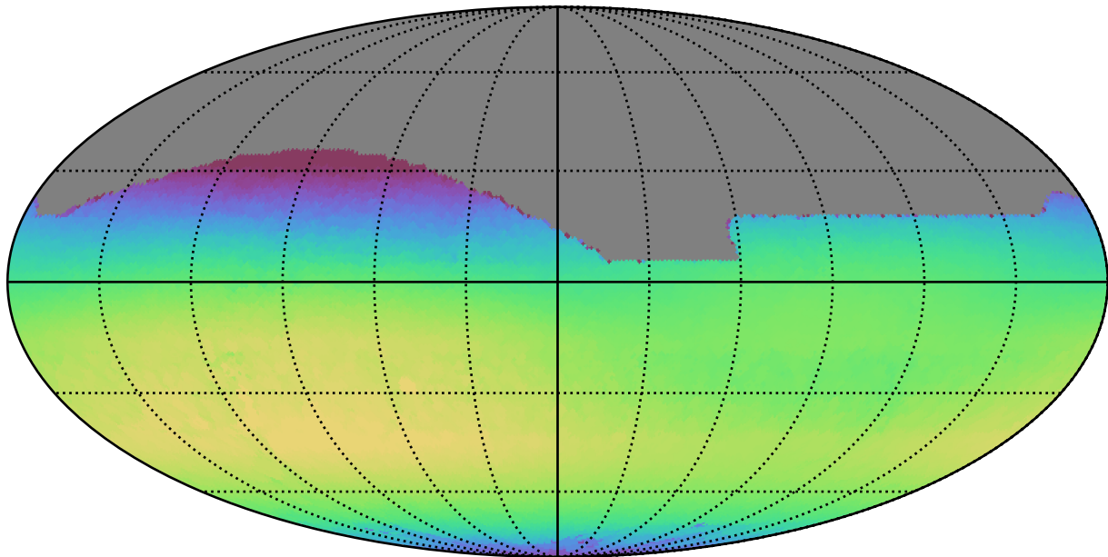
too_elab_r8_d2_giz_v3.4_10yrs All sky i band: Max skyBrightness
