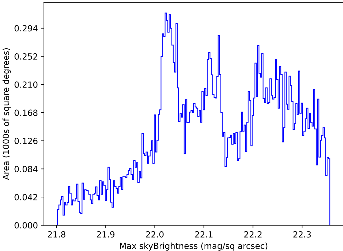
too_elab_r8_d2_giz_v3.4_10yrs All sky g band: Max skyBrightness
