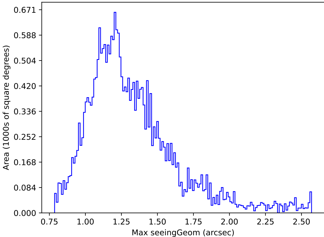
too_elab_r8_d2_giz_v3.4_10yrs Yr 1 z band: Max seeingGeom
