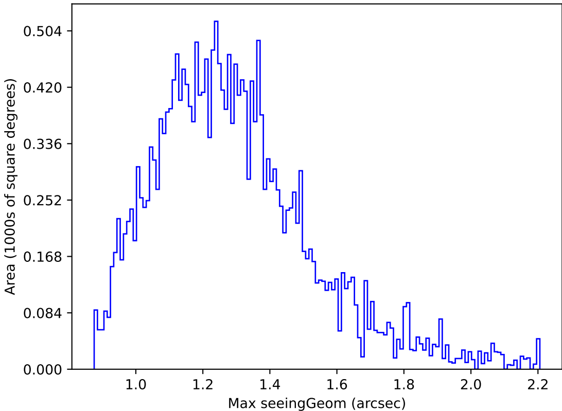
too_elab_r8_d2_giz_v3.4_10yrs Yr 1 y band: Max seeingGeom
