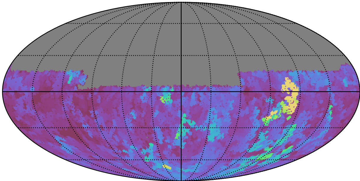
too_elab_r8_d2_giz_v3.4_10yrs Yr 1 u band: Max seeingGeom
