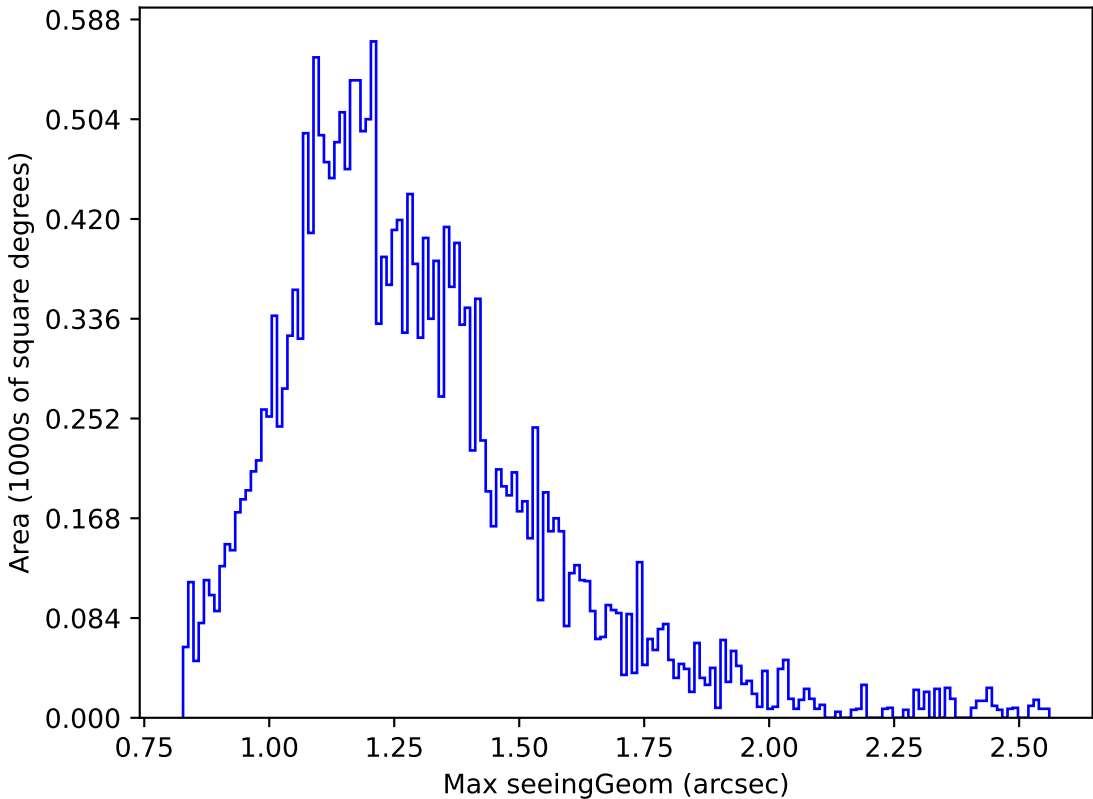
too_elab_r8_d2_giz_v3.4_10yrs Yr 1 u band: Max seeingGeom
