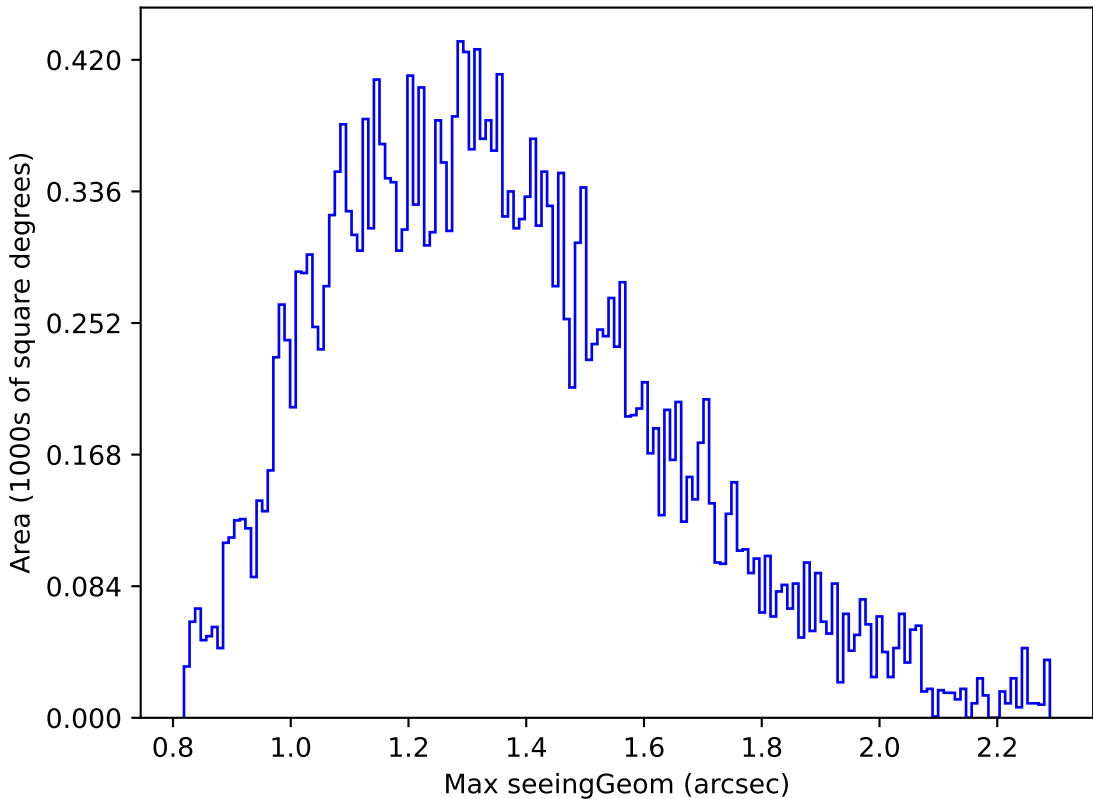
too_elab_r8_d2_giz_v3.4_10yrs Yr 1 r band: Max seeingGeom
