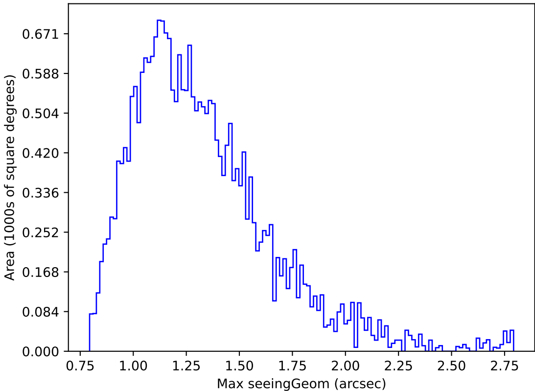
too_elab_r8_d2_giz_v3.4_10yrs Yr 1 g band: Max seeingGeom
