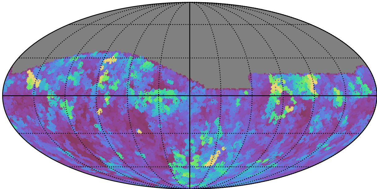
too_elab_r8_d2_giz_v3.4_10yrs Yr 1 all bands: Max seeingGeom
