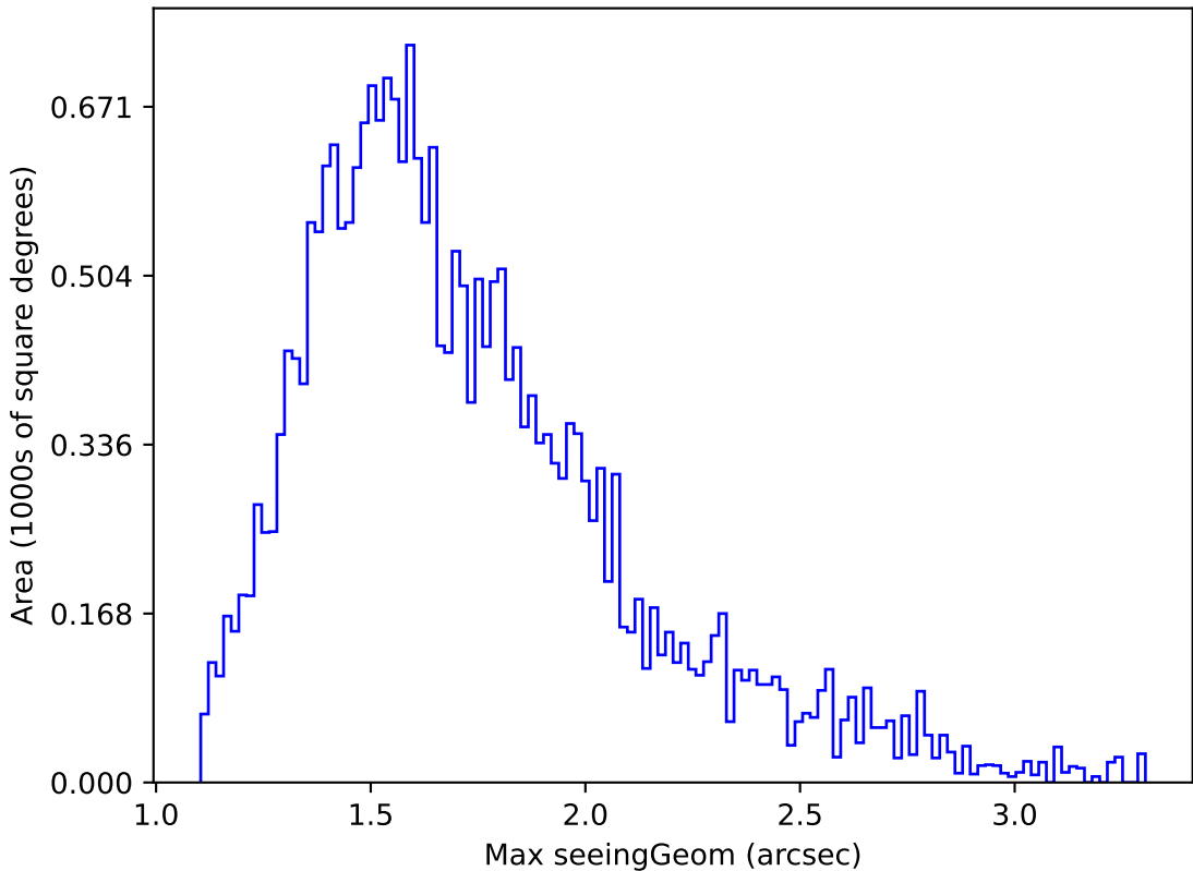
too_elab_r8_d2_giz_v3.4_10yrs Yr 1 all bands: Max seeingGeom
