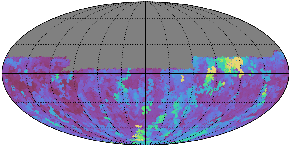
too_elab_r8_d2_giz_v3.4_10yrs Yr 1 u band: Max seeingEff
