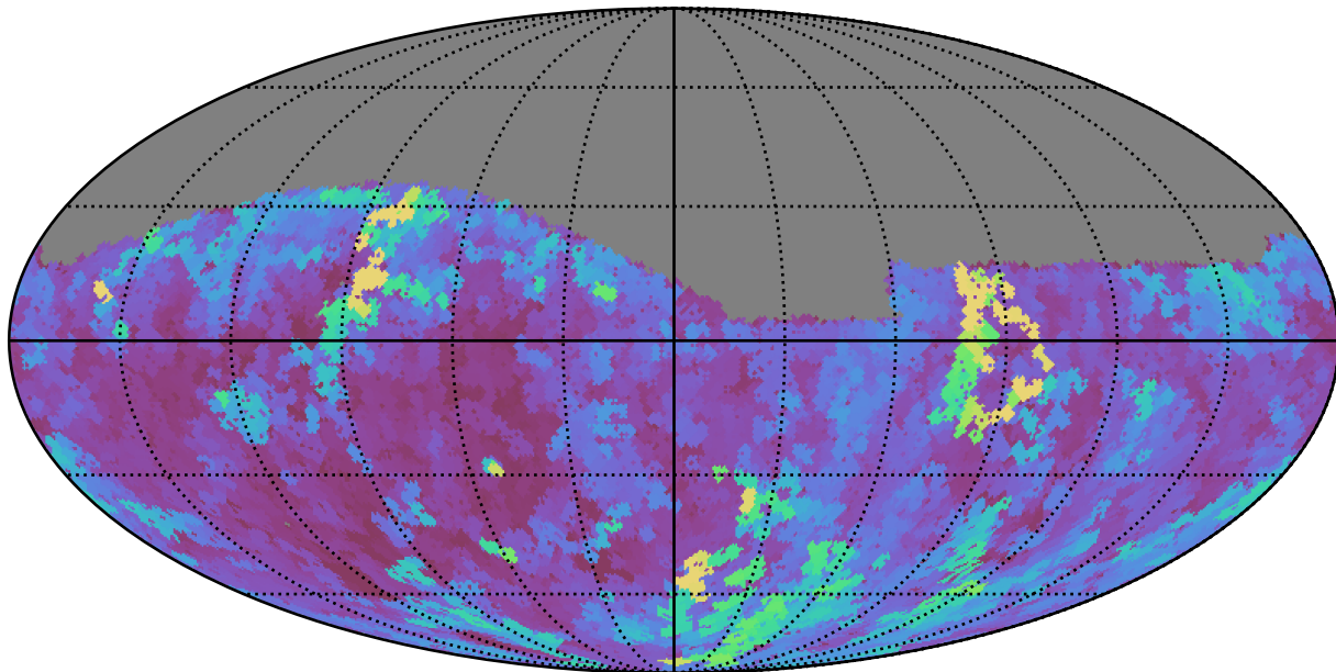
too_elab_r8_d2_giz_v3.4_10yrs Yr 1 g band: Max seeingEff
