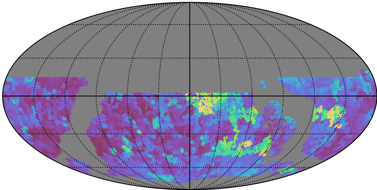
too_elab_r8_d2_giz_v3.4_10yrs WFD y band: Max seeingEff
