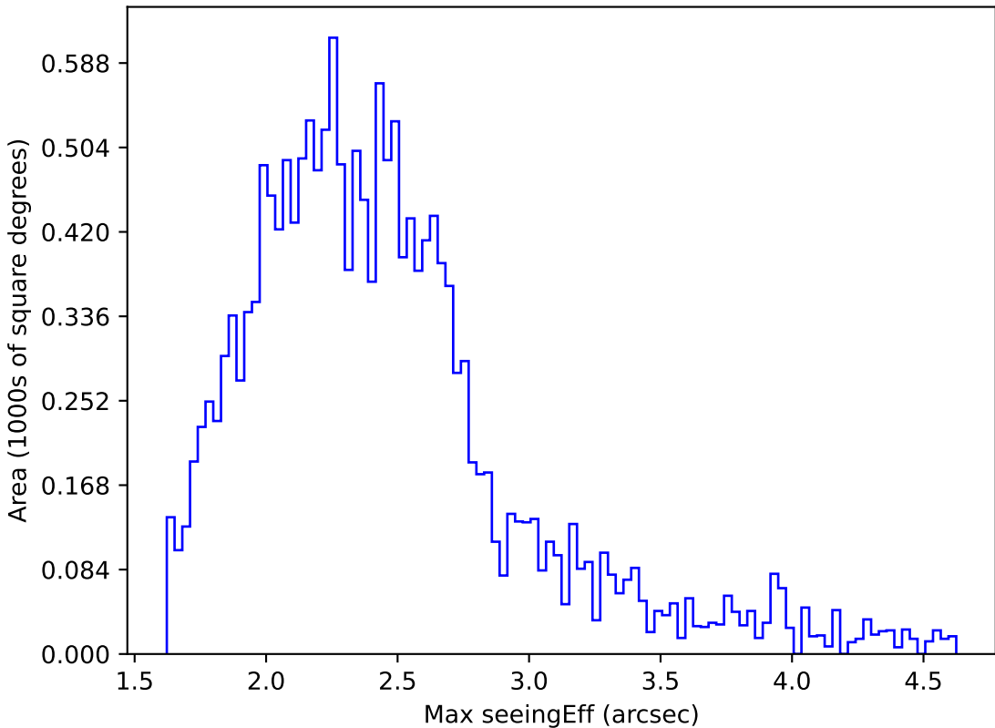
too_elab_r8_d2_giz_v3.4_10yrs WFD y band: Max seeingEff
