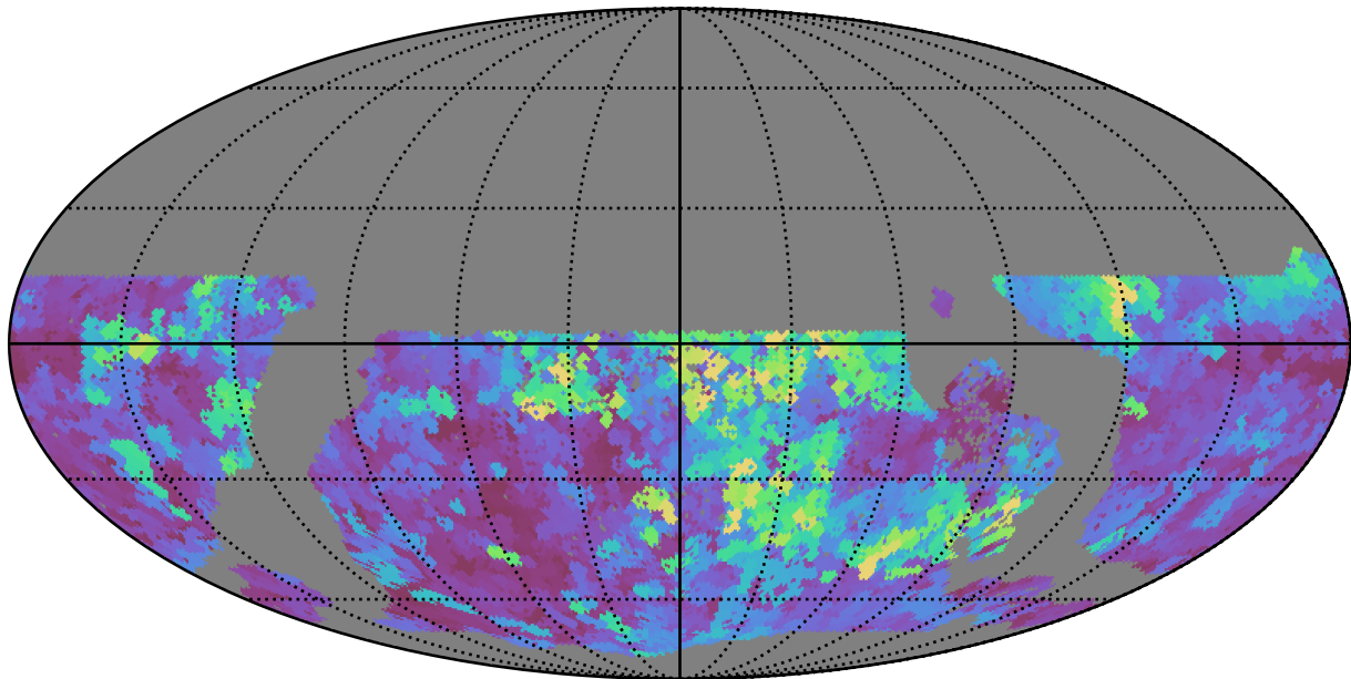
too_elab_r8_d2_giz_v3.4_10yrs WFD u band: Max seeingEff
