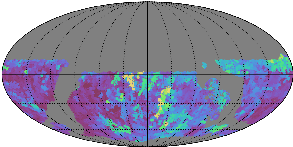
too_elab_r8_d2_giz_v3.4_10yrs WFD r band: Max seeingEff
