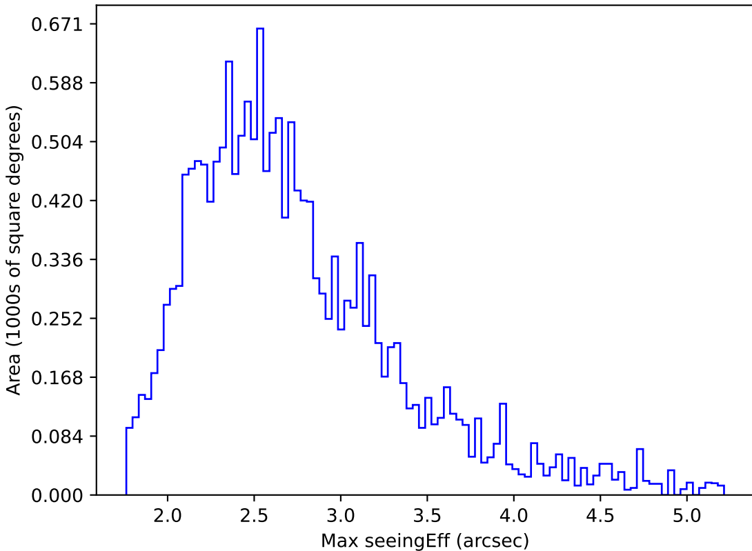
too_elab_r8_d2_giz_v3.4_10yrs WFD i band: Max seeingEff
