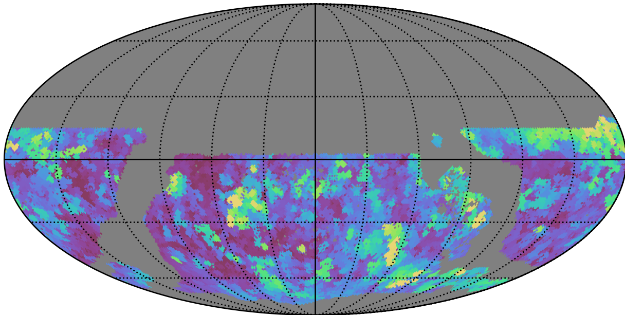
too_elab_r8_d2_giz_v3.4_10yrs WFD g band: Max seeingEff
