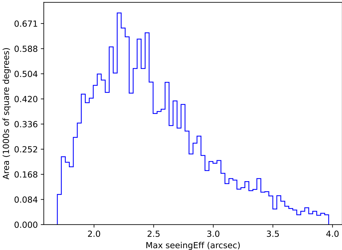
too_elab_r8_d2_giz_v3.4_10yrs WFD g band: Max seeingEff
