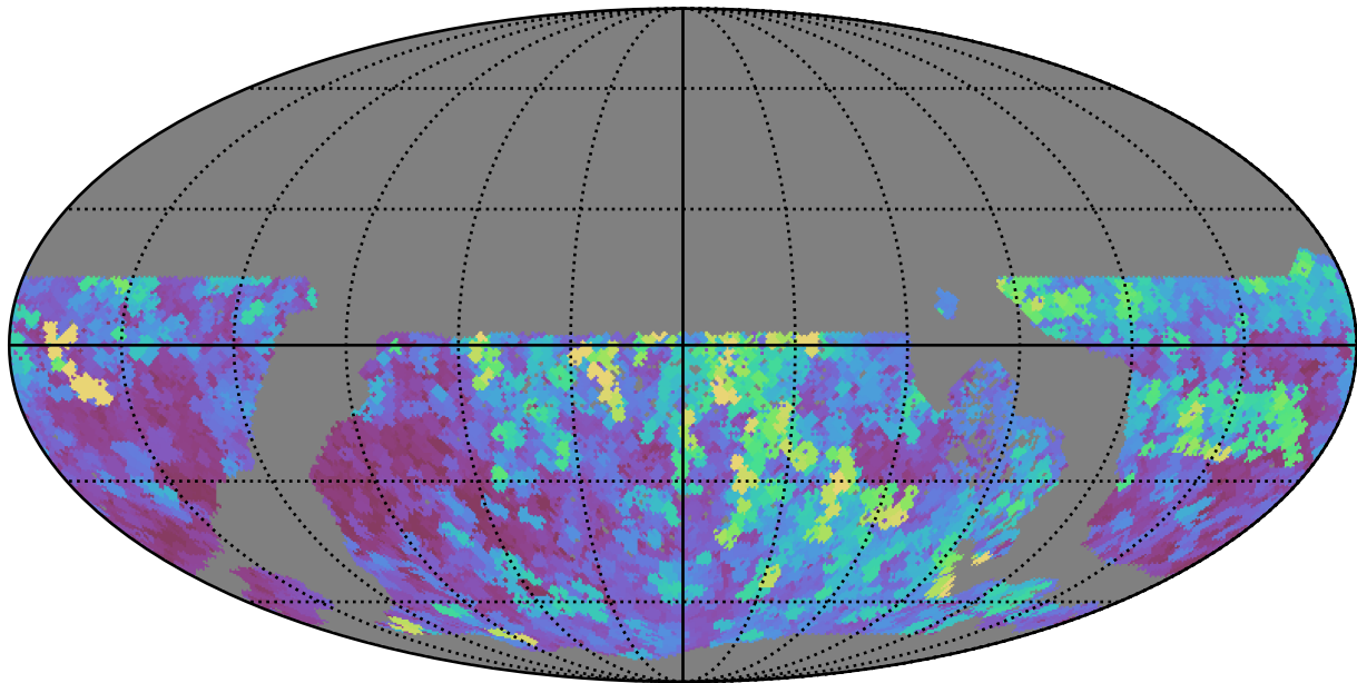
too_elab_r8_d2_giz_v3.4_10yrs WFD all bands: Max seeingEff
