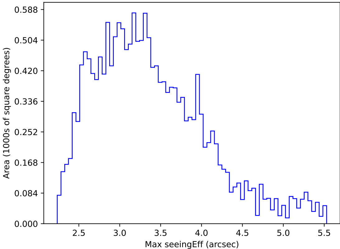
too_elab_r8_d2_giz_v3.4_10yrs WFD all bands: Max seeingEff
