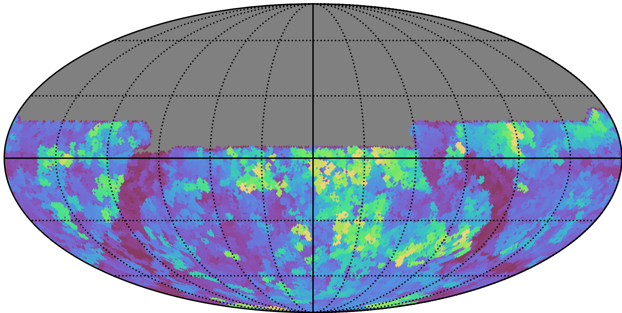
too_elab_r8_d2_giz_v3.4_10yrs All sky u band: Max seeingEff
