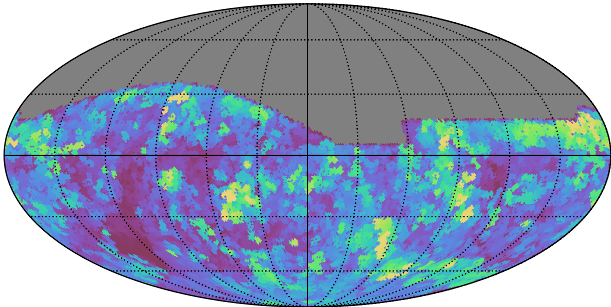
too_elab_r8_d2_giz_v3.4_10yrs All sky g band: Max seeingEff
