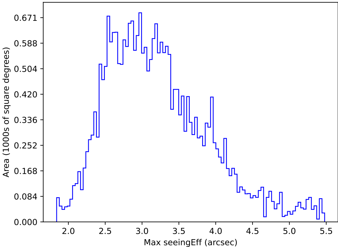
too_elab_r8_d2_giz_v3.4_10yrs All sky all bands: Max seeingEff
