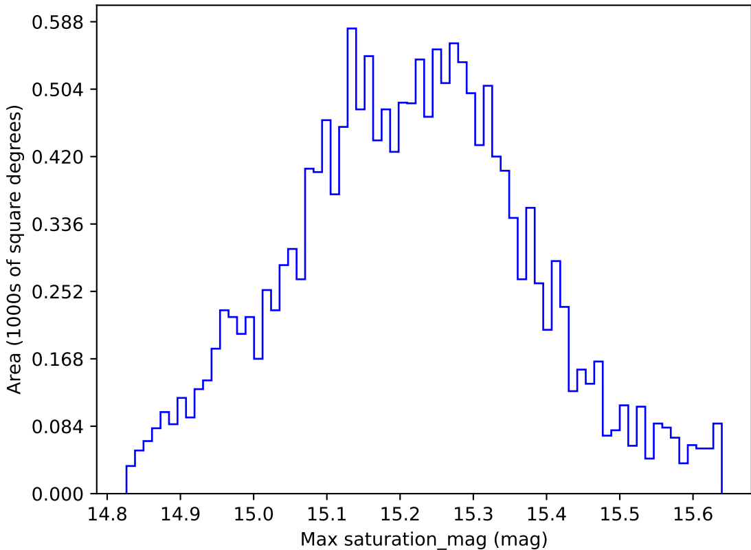
too_elab_r8_d2_giz_v3.4_10yrs WFD z band: Max saturation_mag
