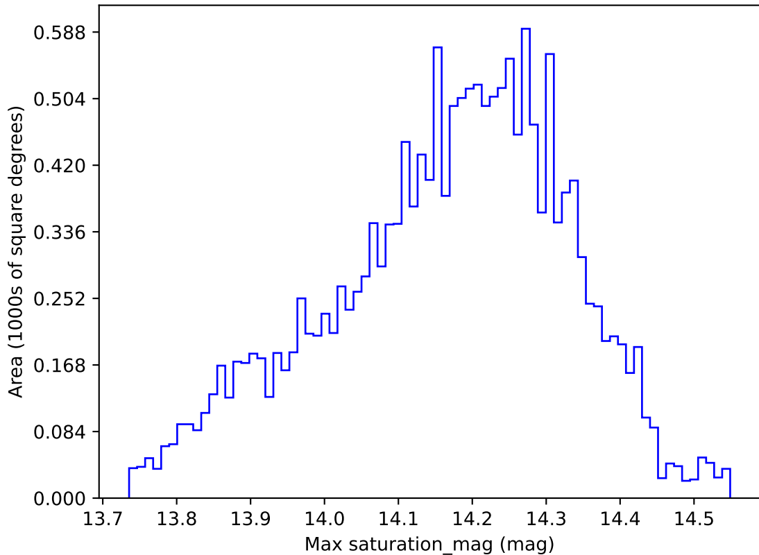
too_elab_r8_d2_giz_v3.4_10yrs WFD y band: Max saturation_mag
