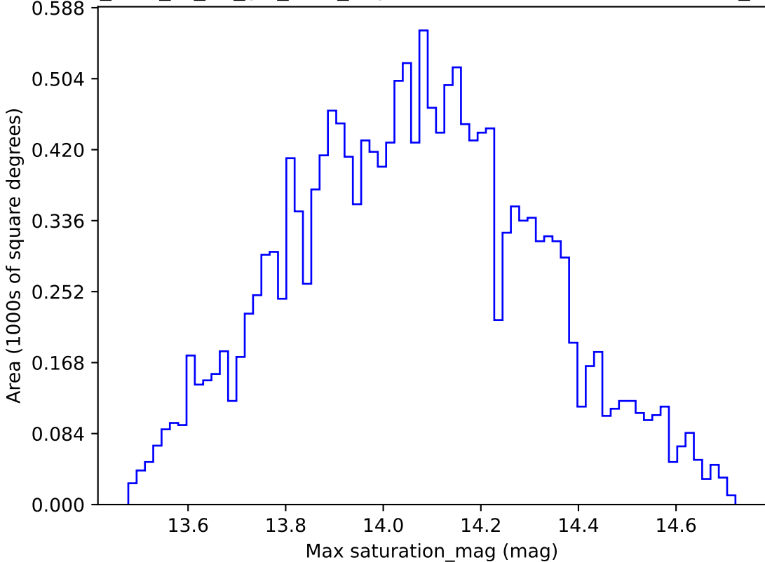
too_elab_r8_d2_giz_v3.4_10yrs WFD u band: Max saturation_mag
