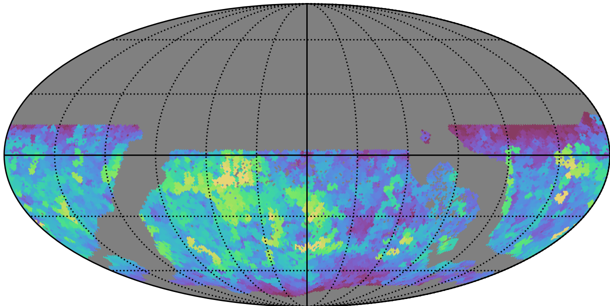
too_elab_r8_d2_giz_v3.4_10yrs WFD r band: Max saturation_mag
