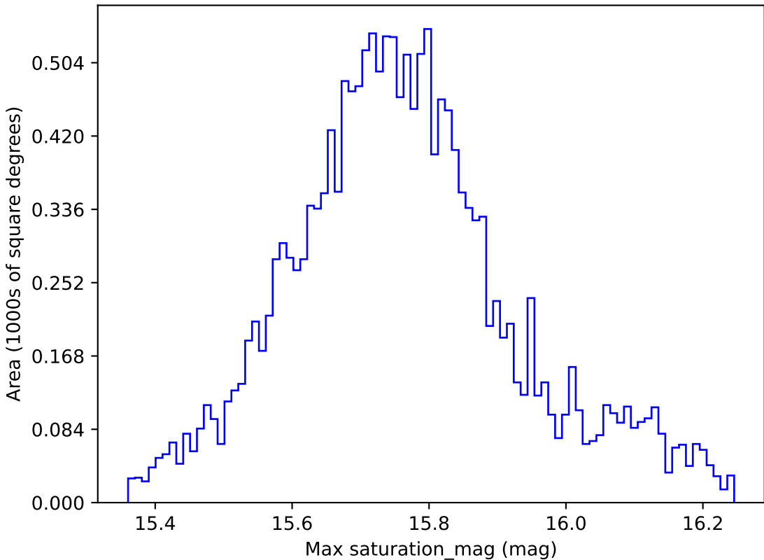
too_elab_r8_d2_giz_v3.4_10yrs WFD r band: Max saturation_mag
