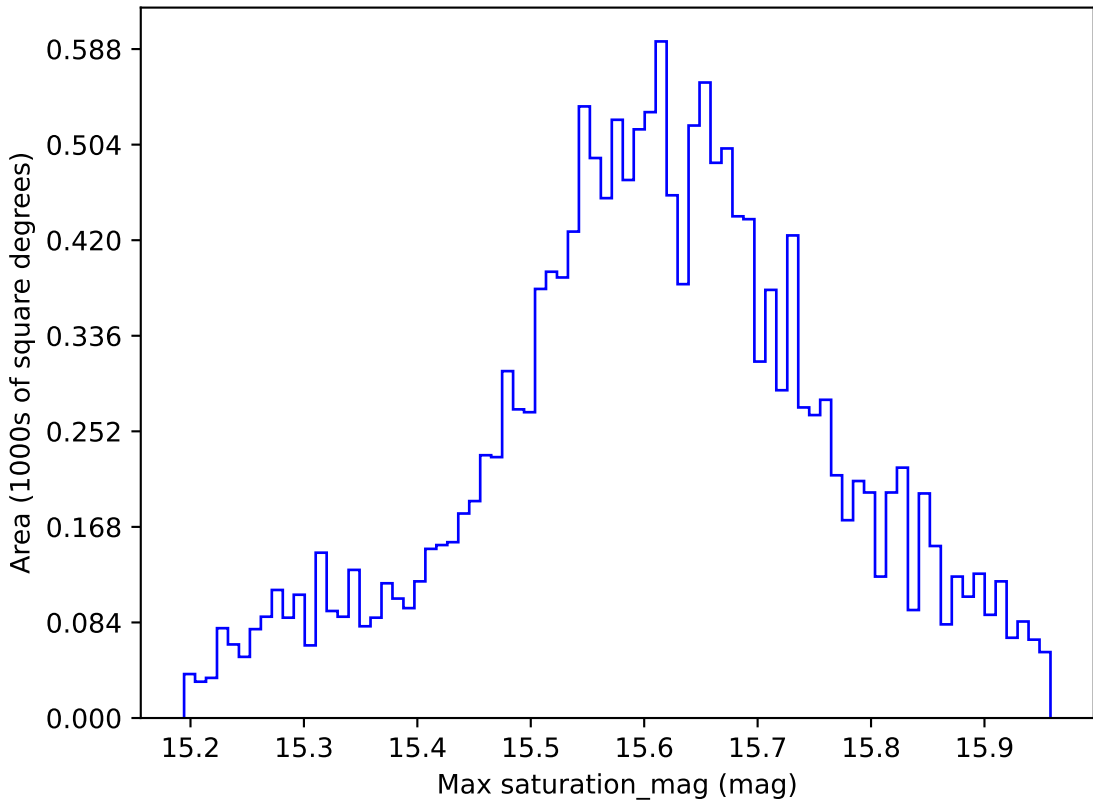
too_elab_r8_d2_giz_v3.4_10yrs WFD i band: Max saturation_mag
