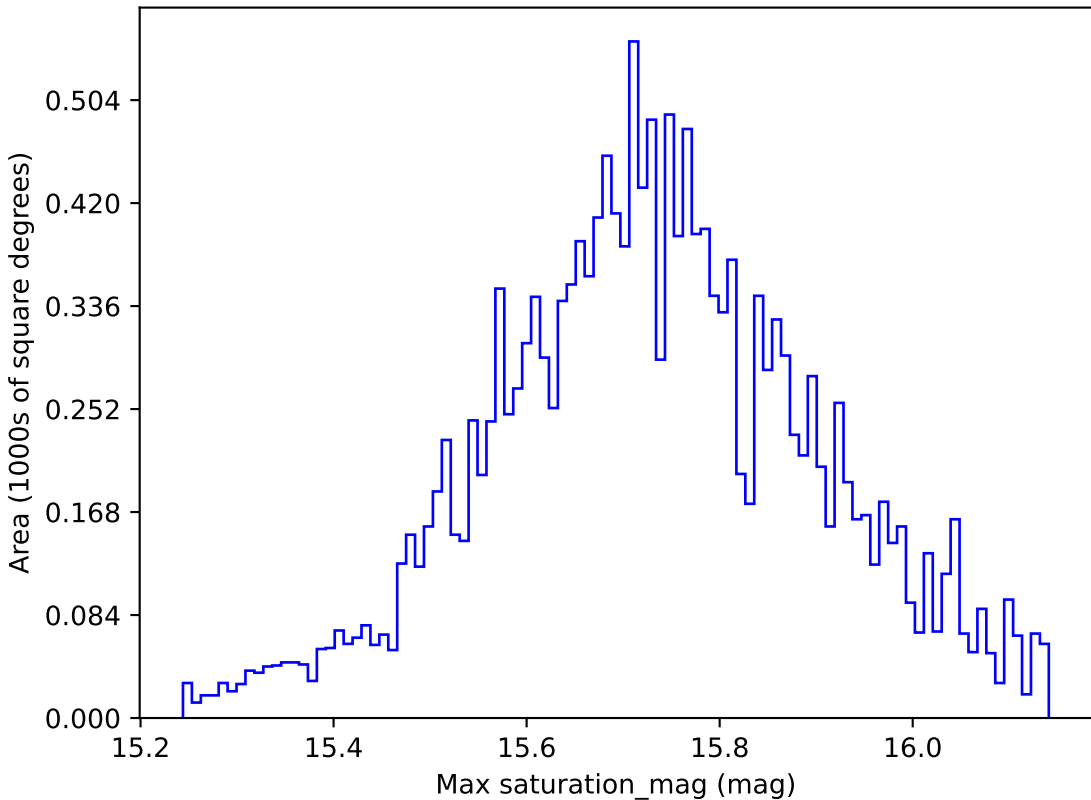
too_elab_r8_d2_giz_v3.4_10yrs WFD g band: Max saturation_mag
