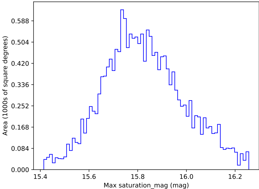
too_elab_r8_d2_giz_v3.4_10yrs WFD all bands: Max saturation_mag
