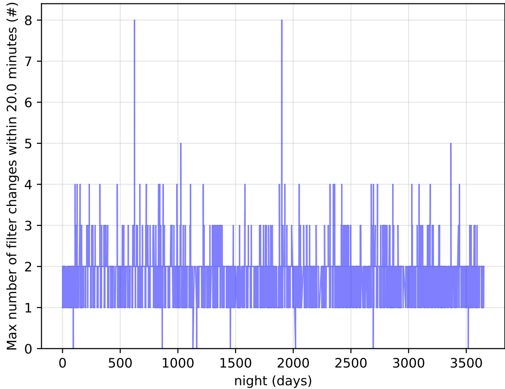
too_elab_r8_d2_giz_v3.4_10yrs Per Night: Max number of filter changes within 20.0 minutes
