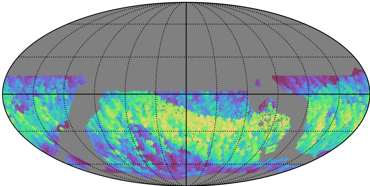
too_elab_r8_d2_giz_v3.4_10yrs WFD z band: Max normairmass
