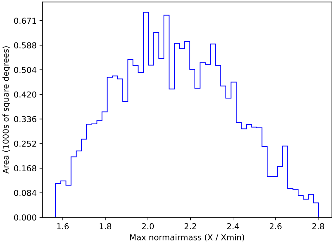
too_elab_r8_d2_giz_v3.4_10yrs WFD y band: Max normairmass
