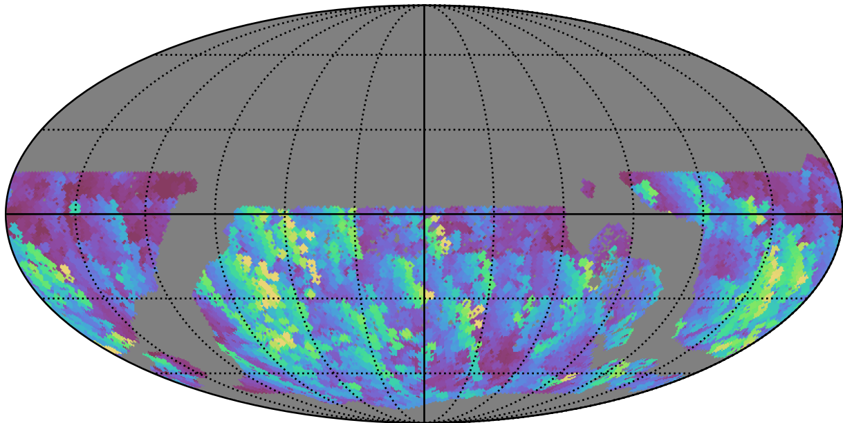
too_elab_r8_d2_giz_v3.4_10yrs WFD u band: Max normairmass
