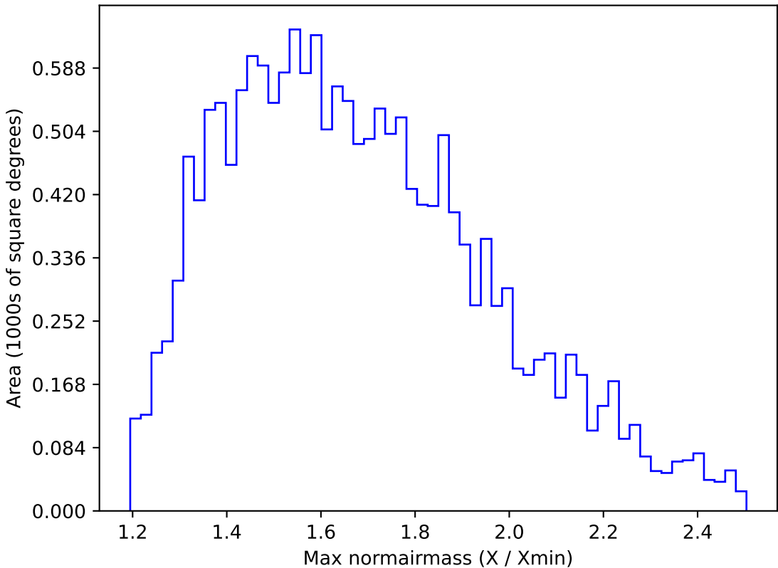
too_elab_r8_d2_giz_v3.4_10yrs WFD u band: Max normairmass
