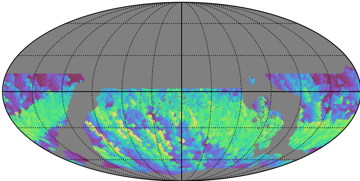
too_elab_r8_d2_giz_v3.4_10yrs WFD r band: Max normairmass
