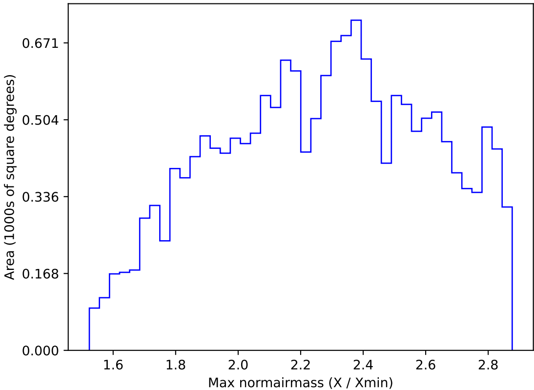
too_elab_r8_d2_giz_v3.4_10yrs WFD i band: Max normairmass
