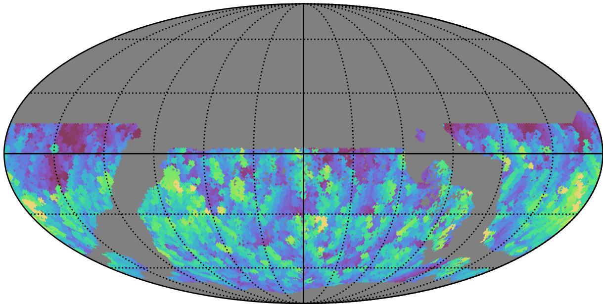
too_elab_r8_d2_giz_v3.4_10yrs WFD g band: Max normairmass
