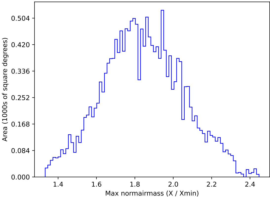
too_elab_r8_d2_giz_v3.4_10yrs WFD g band: Max normairmass
