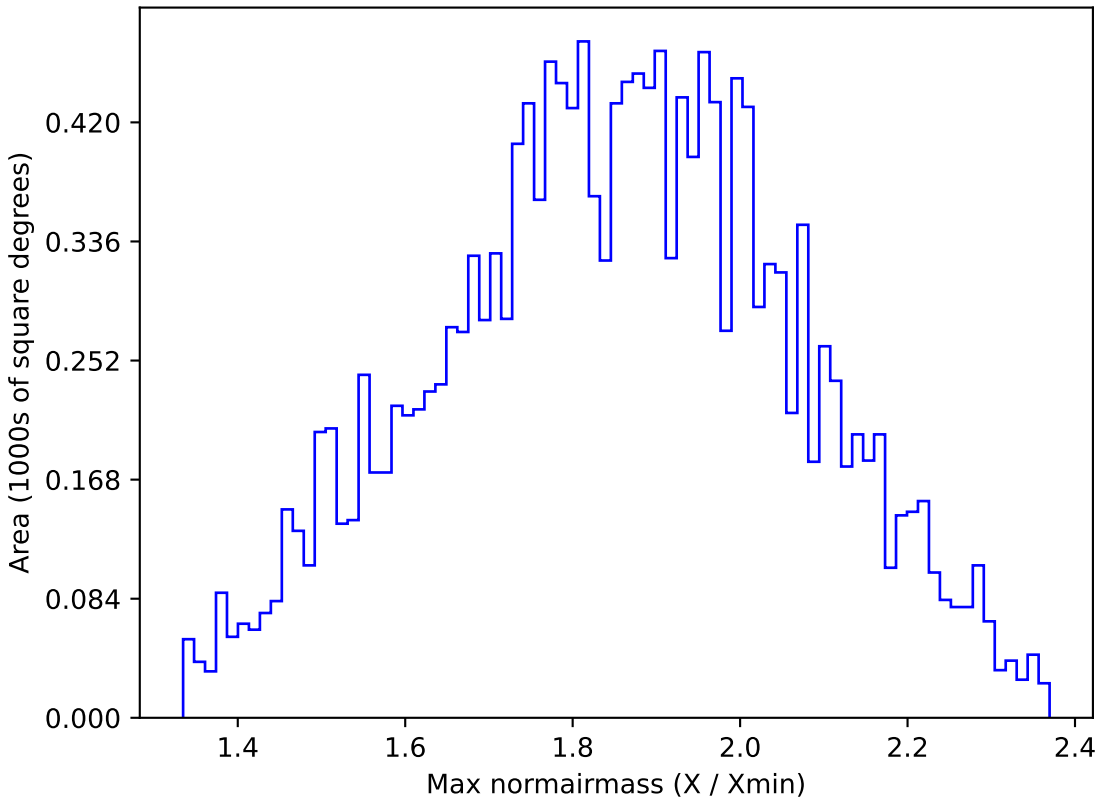
too_elab_r8_d2_giz_v3.4_10yrs WFD g band: Max normairmass
