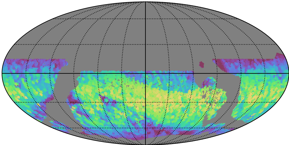
too_elab_r8_d2_giz_v3.4_10yrs WFD all bands: Max normairmass
