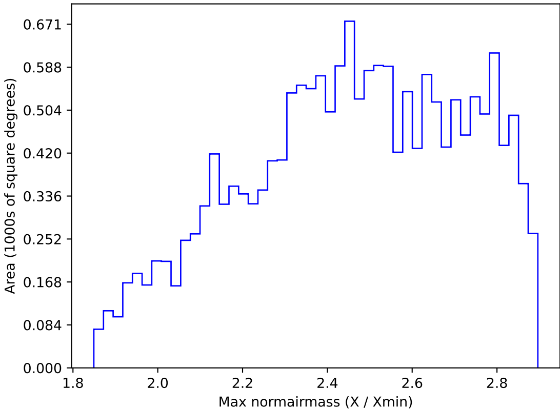
too_elab_r8_d2_giz_v3.4_10yrs WFD all bands: Max normairmass
