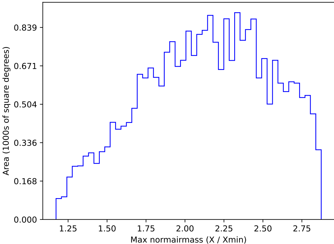
too_elab_r8_d2_giz_v3.4_10yrs All sky z band: Max normairmass
