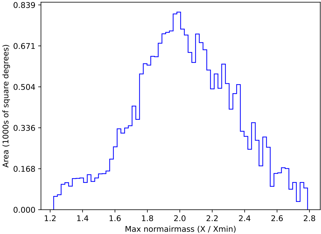
too_elab_r8_d2_giz_v3.4_10yrs All sky y band: Max normairmass
