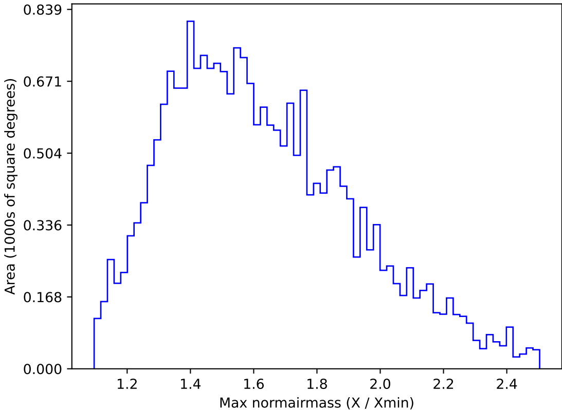
too_elab_r8_d2_giz_v3.4_10yrs All sky u band: Max normairmass
