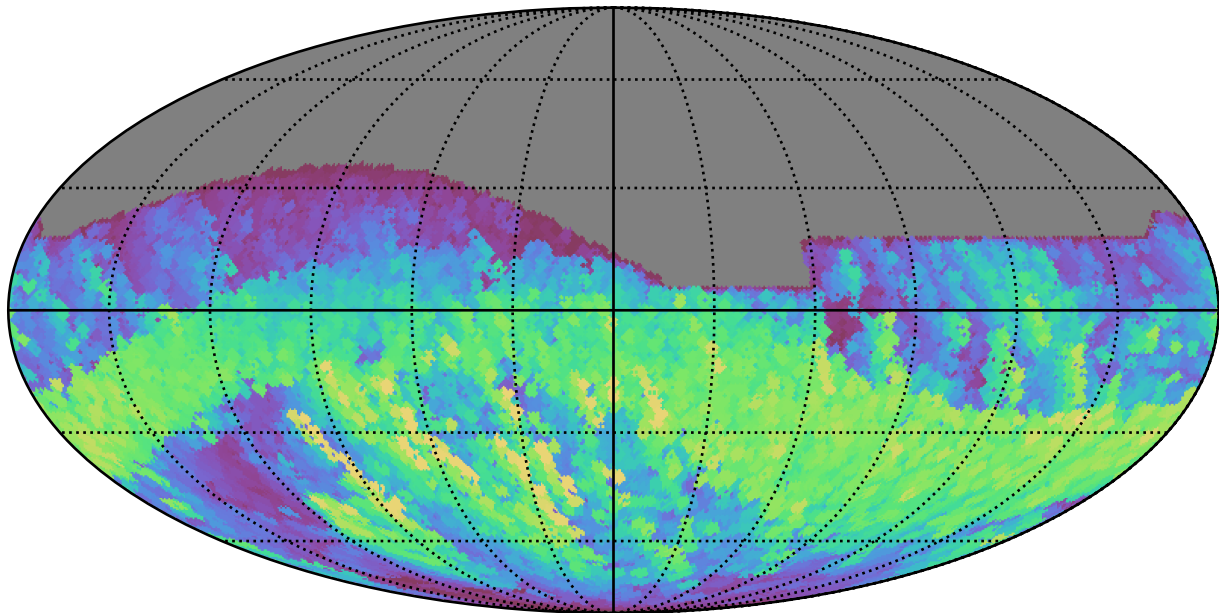
too_elab_r8_d2_giz_v3.4_10yrs All sky r band: Max normairmass
