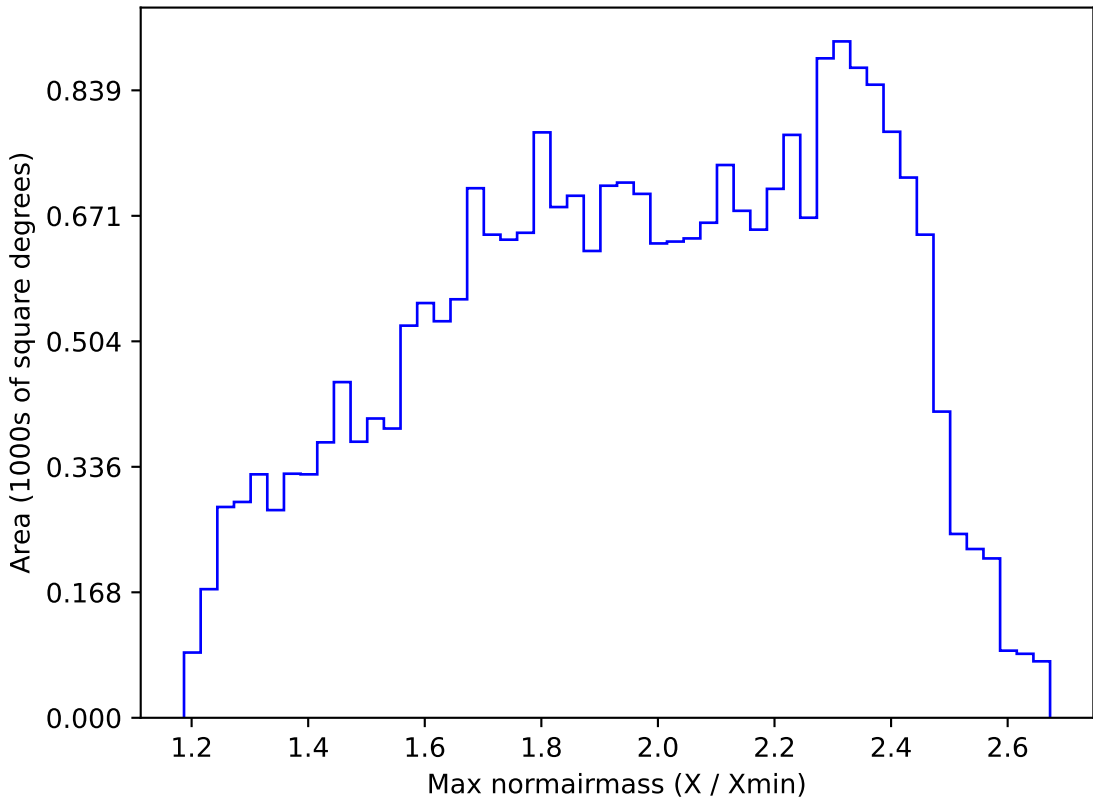
too_elab_r8_d2_giz_v3.4_10yrs All sky r band: Max normairmass
